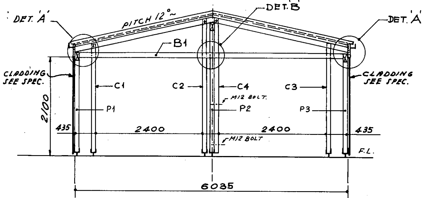
FRONT ELEVATION 1:50
