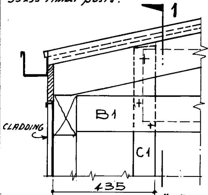
DETAIL "A" 1:10
