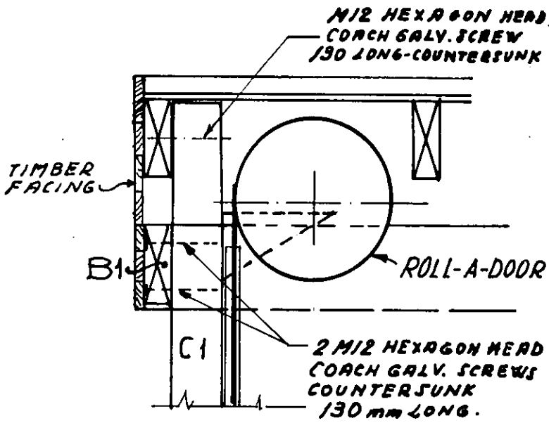
SECTION 1 1:10
