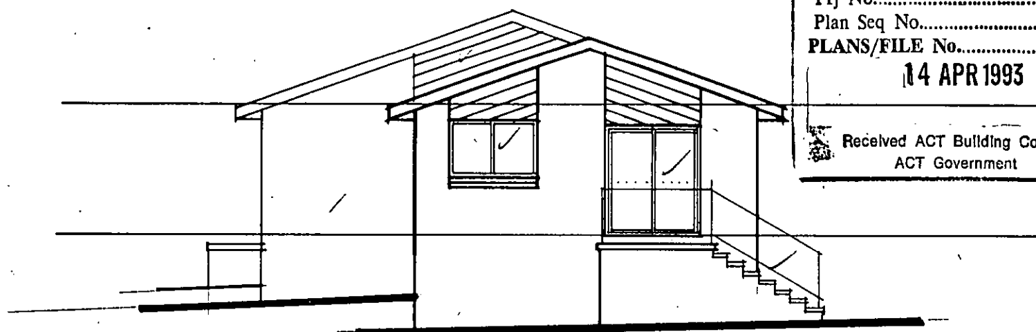
EAST ELEVATION
